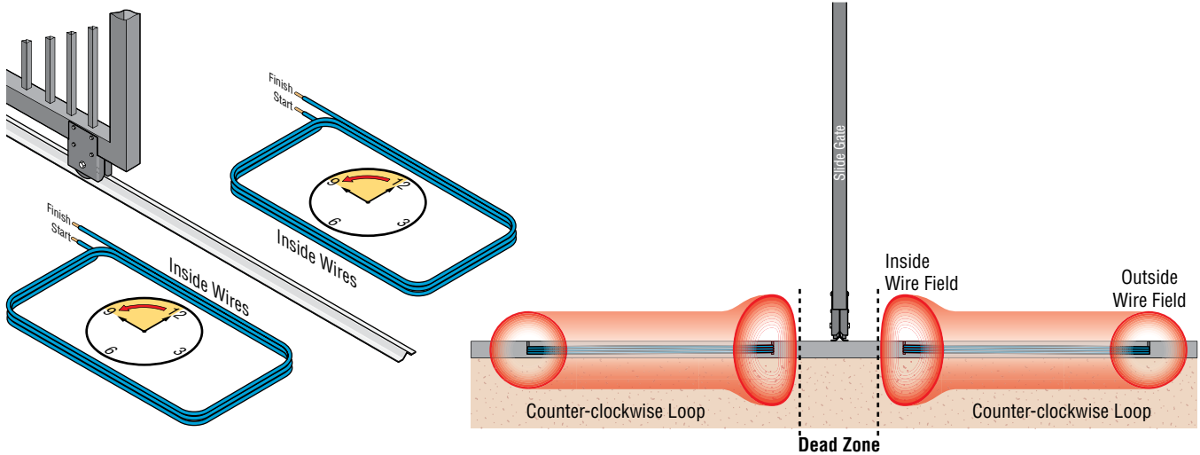
Both loops wound counter-clockwise.
