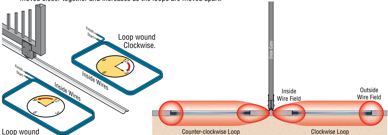
2 loops wound in opposite directions attract the inside wire fields.
