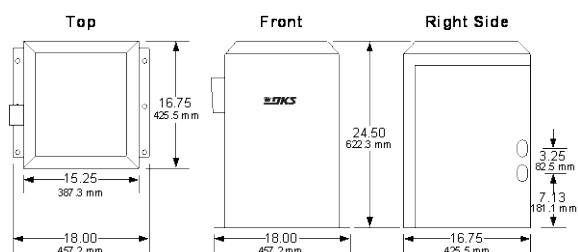
Metal Cover
