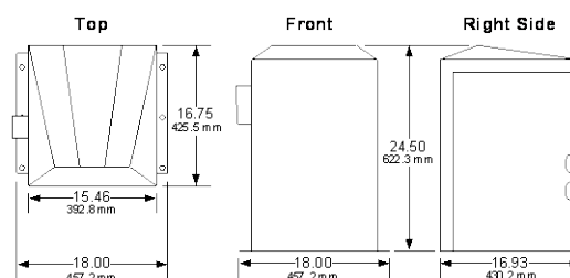
Polypropylene Cover
