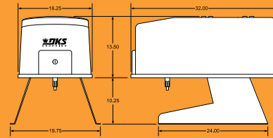
Pad mount adds 10.25" (260mm) to Height dimension.
